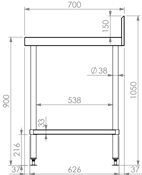
*700mm DEEP MODULE ELEVATION.
