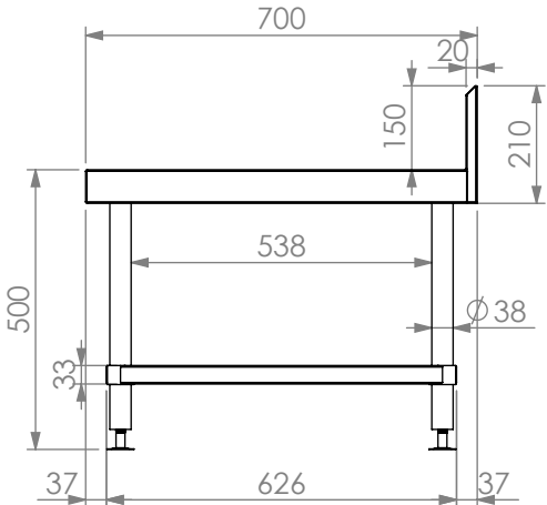
*700mm DEEP MODULE ELEVATION (MIXER STAND).
